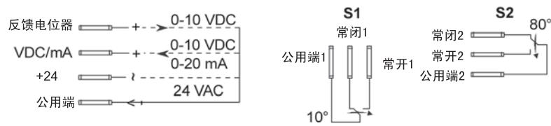
M9109-GGx-4接线图
